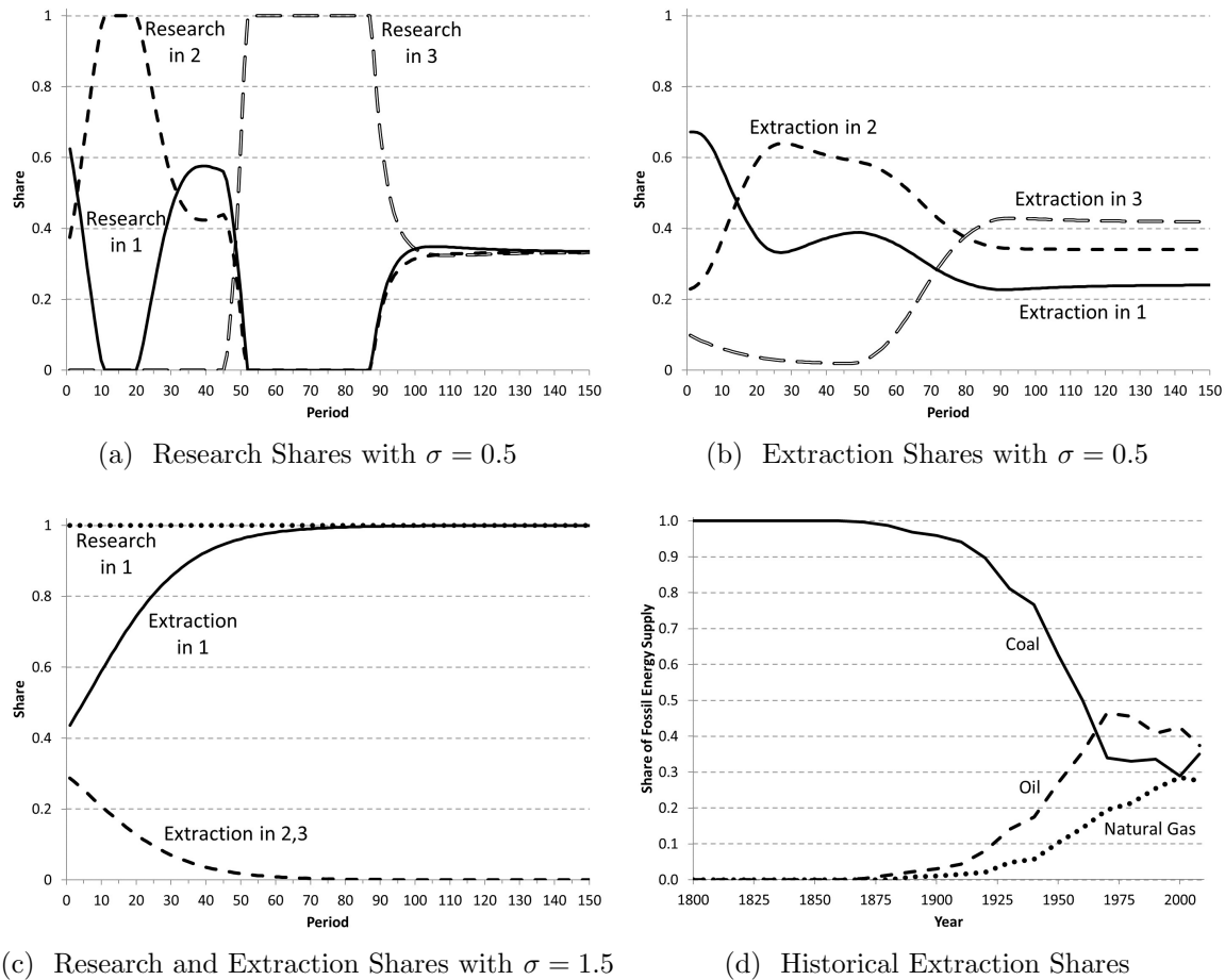
Figure A-1: Top: An example of an innovation-led transition, with \sigma = 0.5 . Bottom left: An example of lock-in, with \sigma = 1.5 . Resources 2 and 3 have nearly identical extraction shares. Bottom right: Shares of global fossil energy supply, from Smil (2010).
